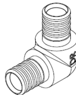
ISOMETRIC VIEW SCALE 1:1
